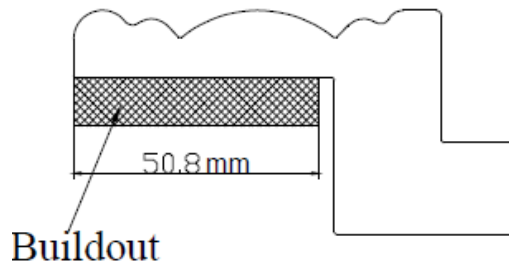
Crown Z Frame 76mm
