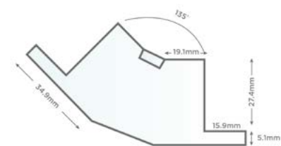
(Deco Frame) 32mm with insert
