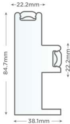
Double Insert F Frame 84mm
