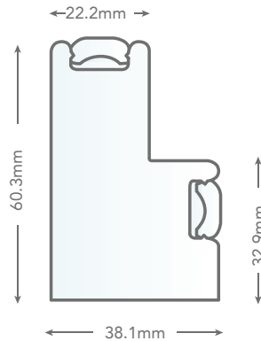
Double Insert L Frame 60mm
