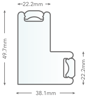
Double Insert L Frame 50mm
