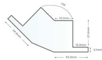
(Deco Frame) 32mm
