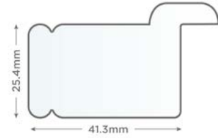
41.3mm D-Mould Stile
