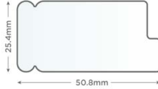
50.8mm Rebate Stile
