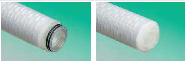
Code 2 = 226/FLAT + Locks
