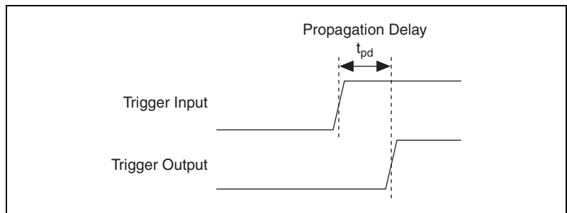
Figure 3-8. Asynchronous Routing Operation
