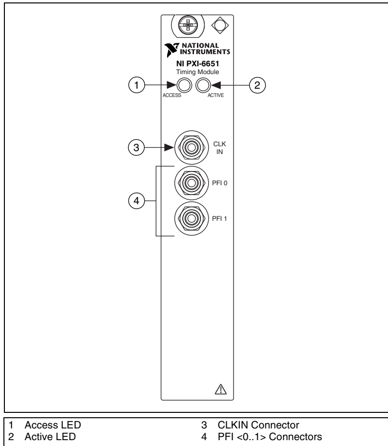
Figure 3-5. NI PXI-6651 Front Panel
