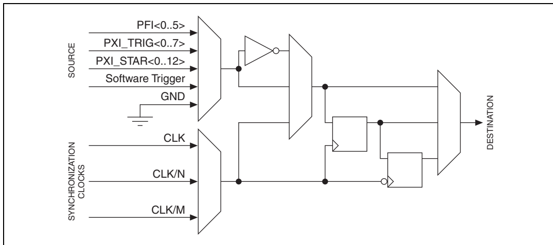
Figure 3-7. Signal Selection Circuitry Diagram
