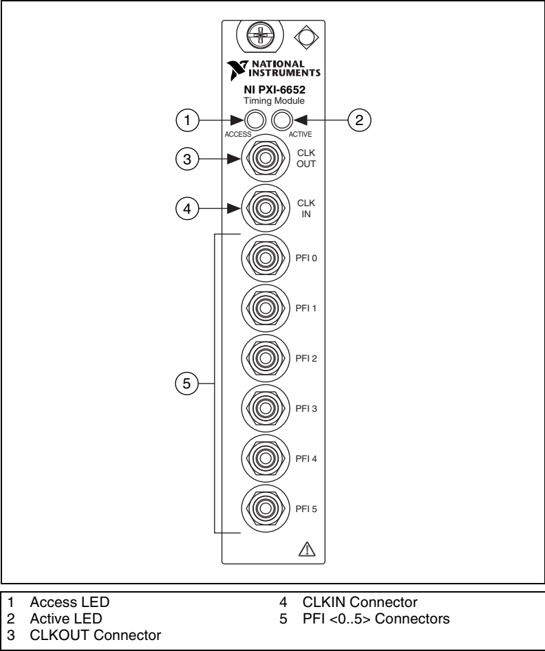
Figure 3-4. NI PXI-6652 Front Panel
