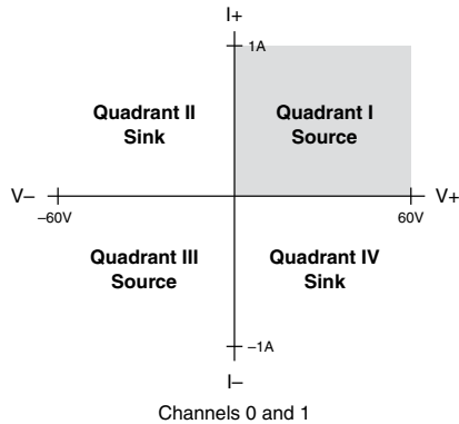
Figure 1. NI 4112 Quadrant Diagram
