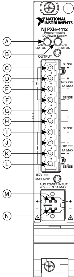
Figure 3. Front Panel
