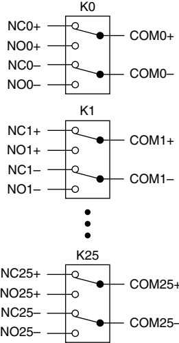
Figure 1. NI PXI-2523 Hardware Diagram
