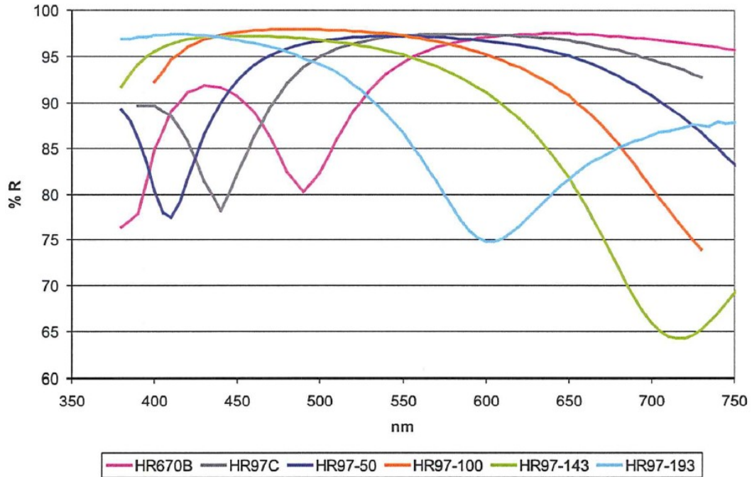
97% R High Reflector Family
