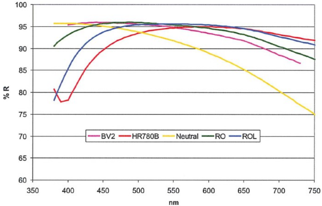
94% R High Reflector Family
