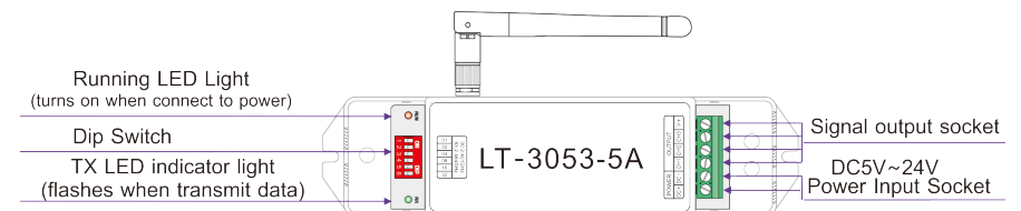
LT-3053-5A wireless receiver
