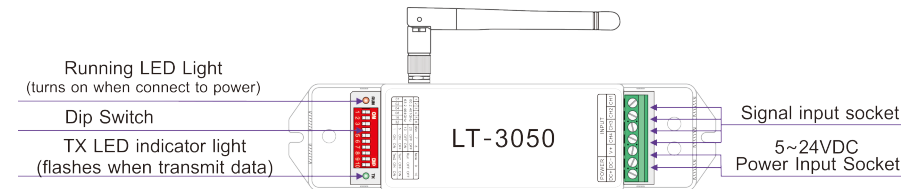
LT-3050 wireless transmitters
