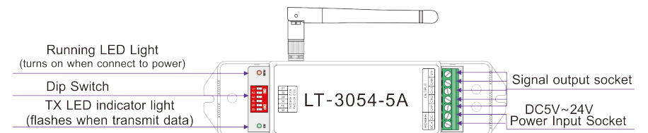
LT-3054-5A wireless receiver
