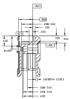
SECTION C-C
