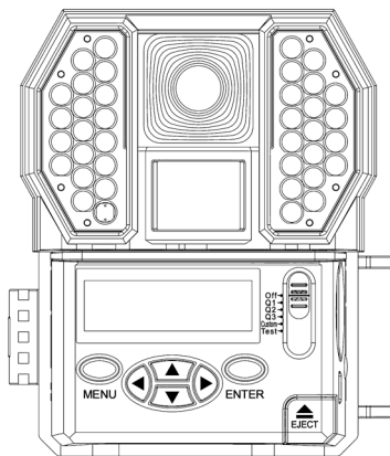
Front Open
