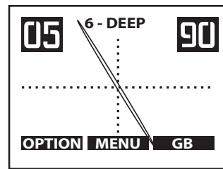
Typical signature for rejected ferrous.
