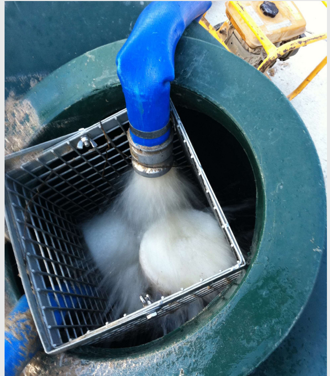
Dam water recirculation using pumps and a 1,000 litre tank
