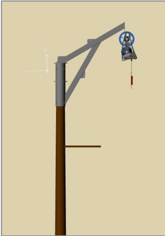
Figure 73 POWERFAN® mounted below supporting structure.
