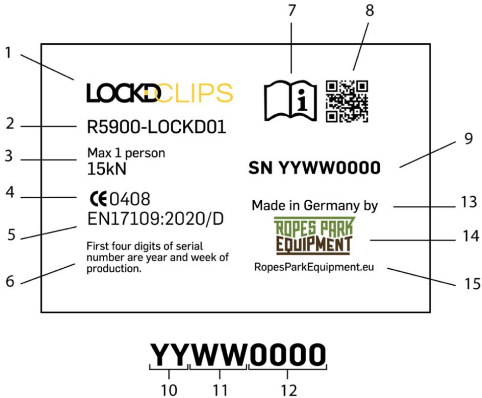
Figure 7: Identification label and serial number
