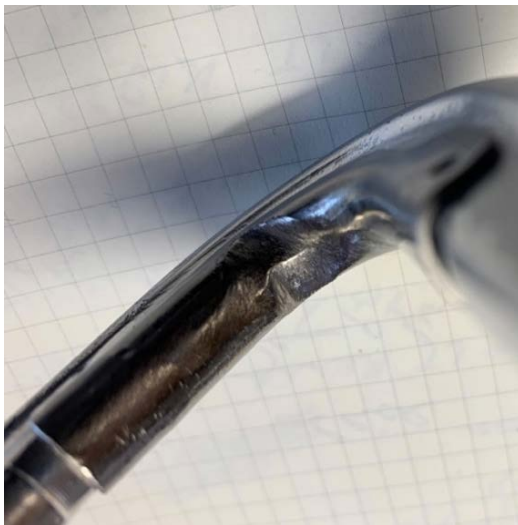
Figure 22:: Slightly worn abrasion guard - does not require replacement
