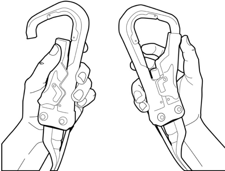
Figure 16: Opening the unlocked hook by pressing on the carabiner gate, the second carabiner remains locked
