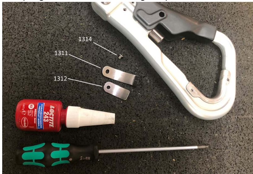
Figure 19: Components of the gate spring
