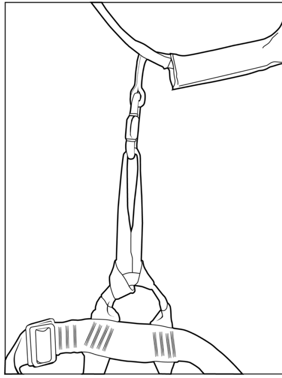
Figure 15: Connection to harness with maillon rapide and lanyard
