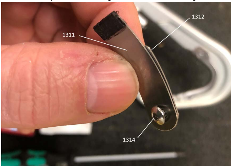
Figure 20: Positioning of the two springs one behind the other
