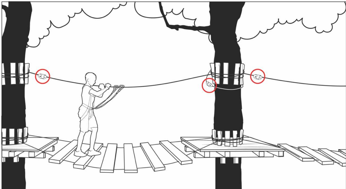
Figure 18: Life Safety Ropes of a Ropes Course with Tweezles Installed
