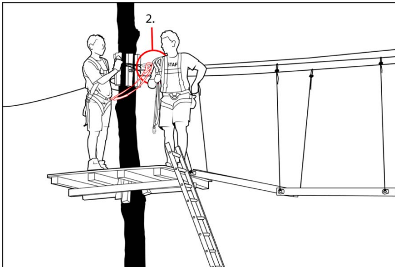
Figure 28: Replacement LockD Clips system to be installed with non-functioning system still connected
