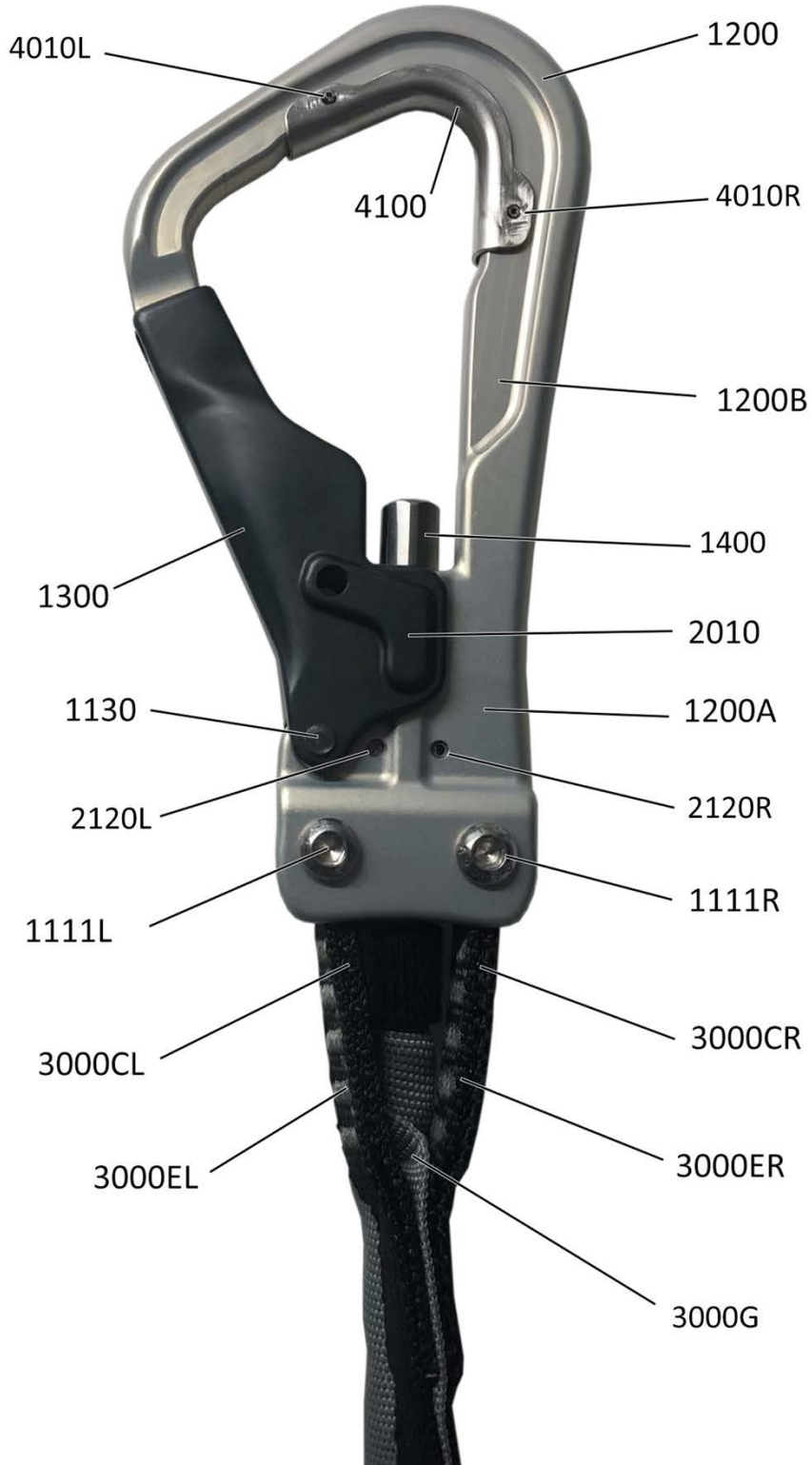
Figure 4: Carabiner Head
