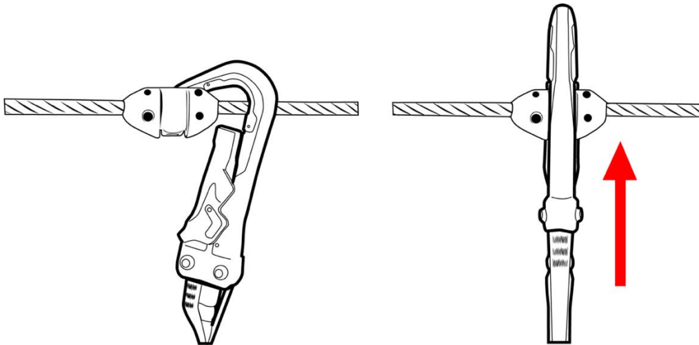
Figure 17: Tweezeling an unlocked carabiner head
