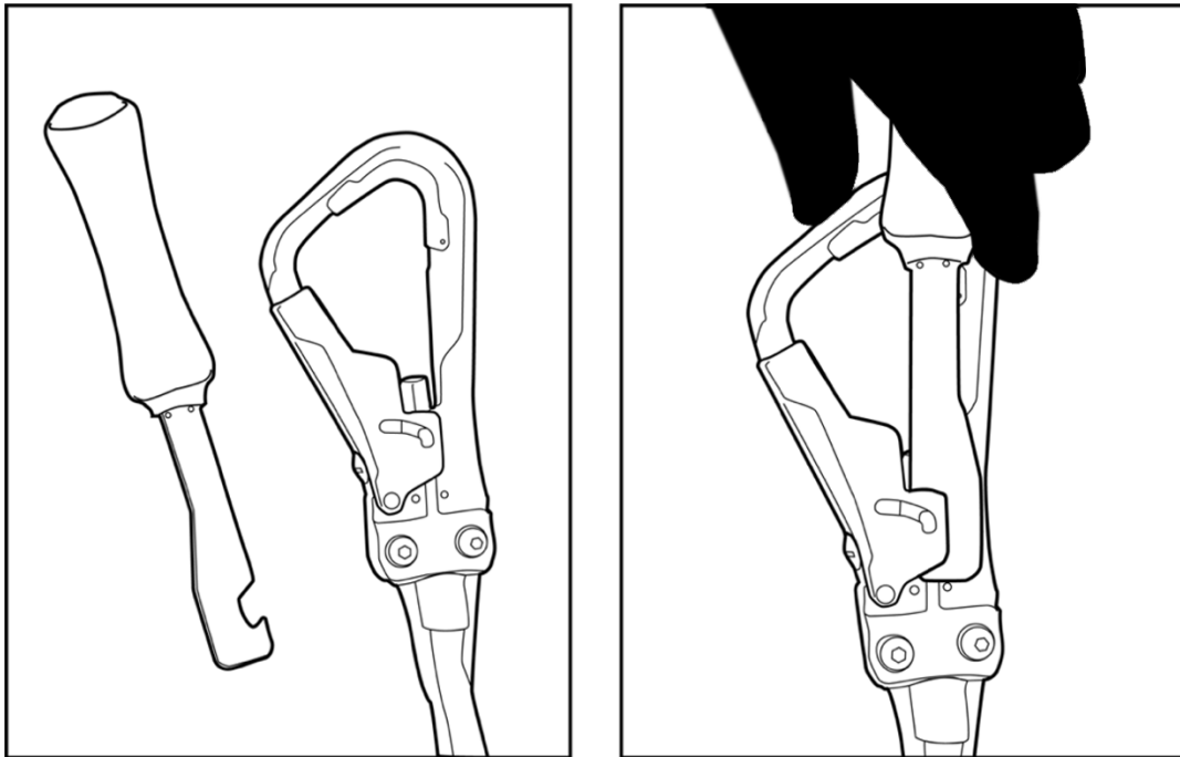
Figure 30: Use of the Carabiner Removing Tool with safety gloves
