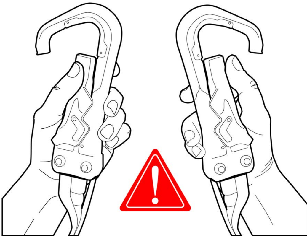
Figure 25: Alpha error
