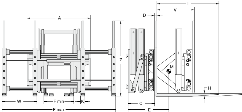
Multi Pallet Handler - Shaft Guide Concept (press the icon)
