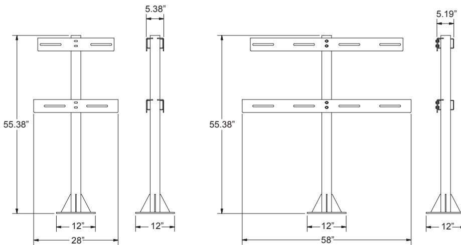
Back-to-back mounting
