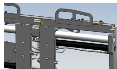
Protection of hydraulics connection (for Types 06/09/10 only)
