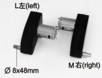
驱动波箱 Drive gearbox
