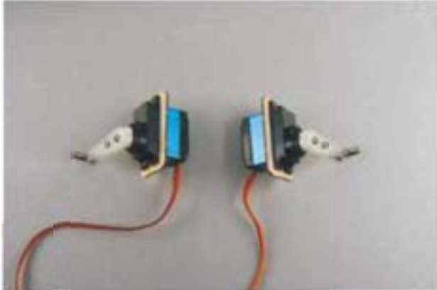
9. Install the servo mounts as picture shown.
