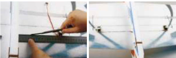
20. Use knife to cut slots on wing, then embed aileron servo leads as picture shown.
