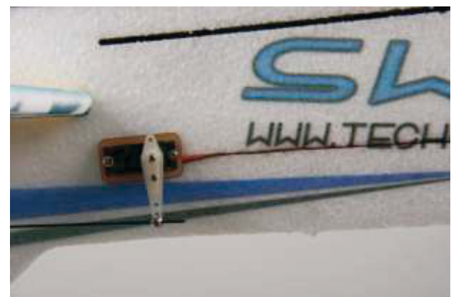
33. Embed the rudder and elevator servo leads into the pre-cut slots on two sides of fuselage. Pls use the servo extension wire if the servo wire is not long enough.
