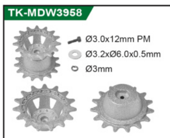
金属驱动轮(含螺丝、弹垫) Metal driving wheel(Included screws, spring mat)
