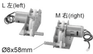
驱动波箱(塑胶齿轮) Drive gearbox ( Plastic gear )
