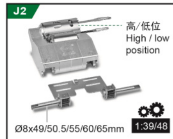
双流驱动波箱 Dual-current drive gear box
