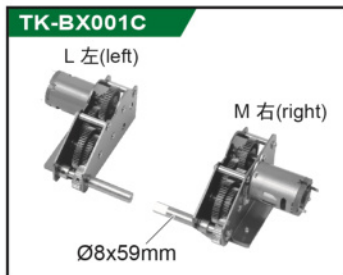
终极版驱动波箱(全轴轴承、钢质齿轮) Ultimate edition drive ultimate box ( Full shaft bearing, Steel gear)
