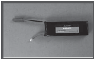
DY-6016 14.8V 4000mAh 25C Li-Po Battery
