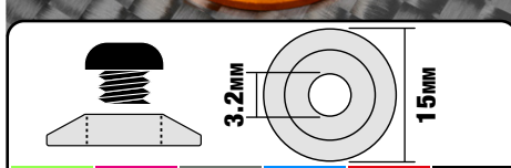
WASHER FOR BUTTON HEAD SCREW ALUMINIUM - 10 PCS
