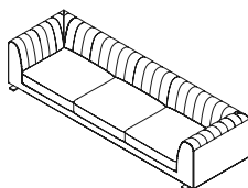
W 260cm D 80cm H 68cm Seat H 41cm
