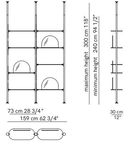
Bookcase composition with 2 units - version "B"
