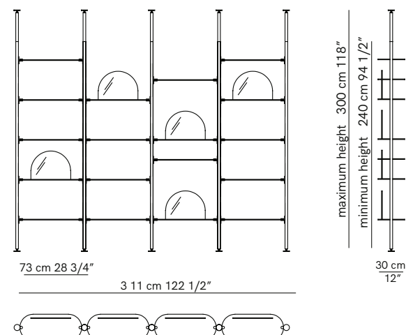
Bookcase composition with 4 units - version "B"
