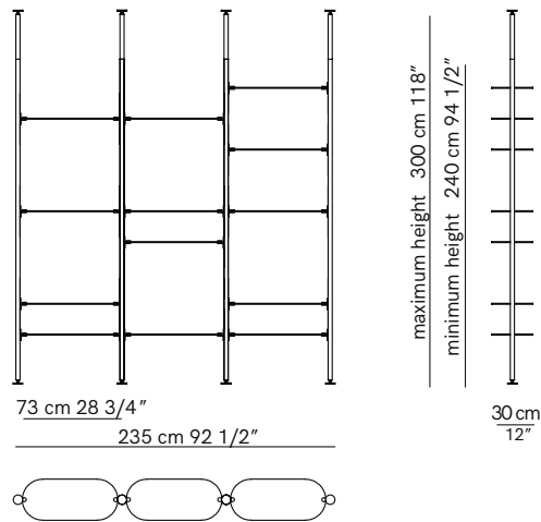
Bookcase composition with 3 units - version "A"
