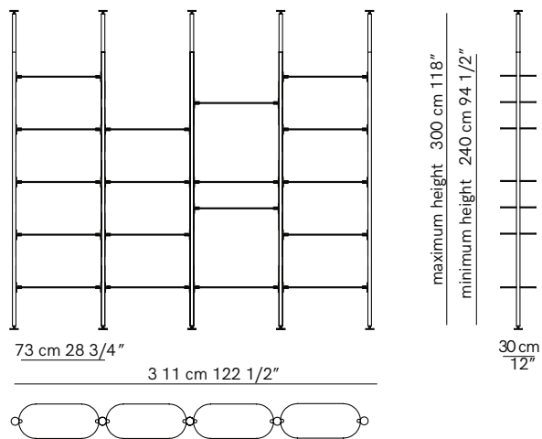
Bookcase composition with 4 units - version "A"
