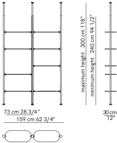
Bookcase composition with 2 units - version "A"
