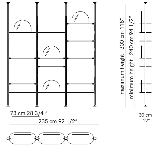
Bookcase composition with 3 units - version "B"
