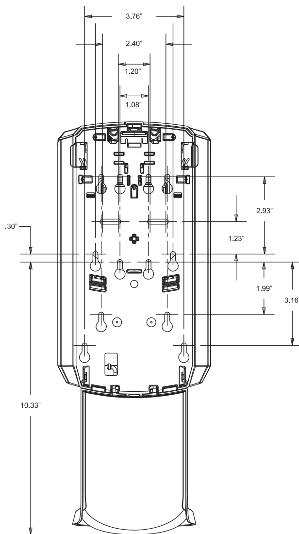
Back View
