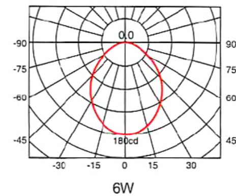
The light intensity distribution curve of polar coordinate
