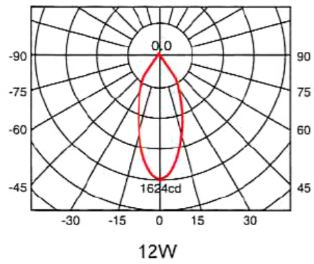
The light intensity distribution curve of polar coordinate
