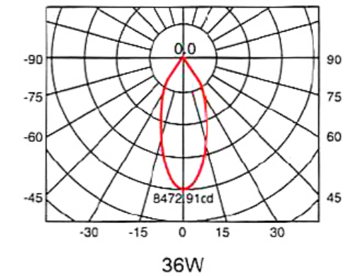
The light intensity distribution curve of polar coordinate
