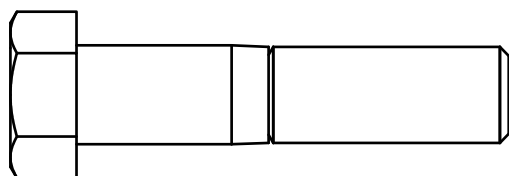
(A2)HEX BOLT 1/2"x2 1/4"L PARTIAL THREAD QTY.8
