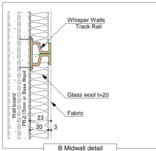
B Midwall detail
