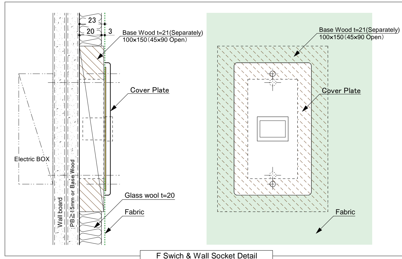
F Switch & Wall Socket Detail
