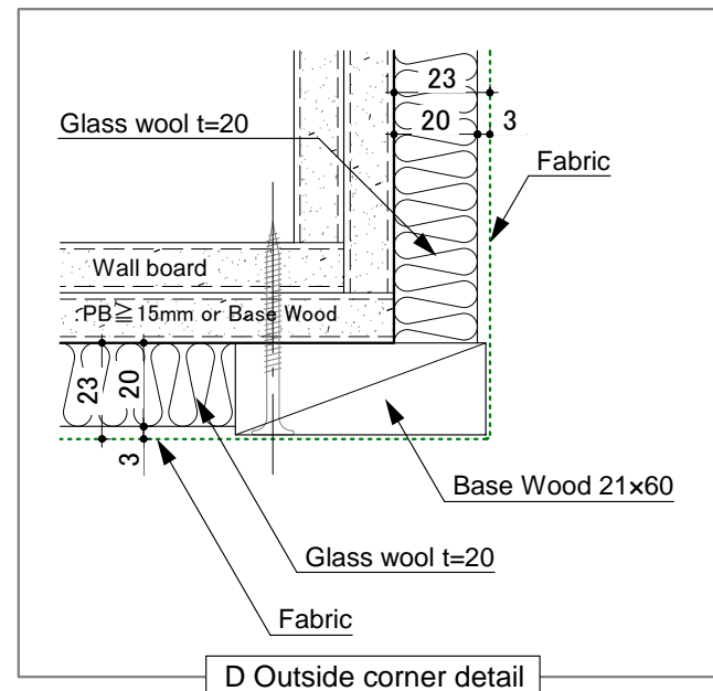
D Outside corner detail
