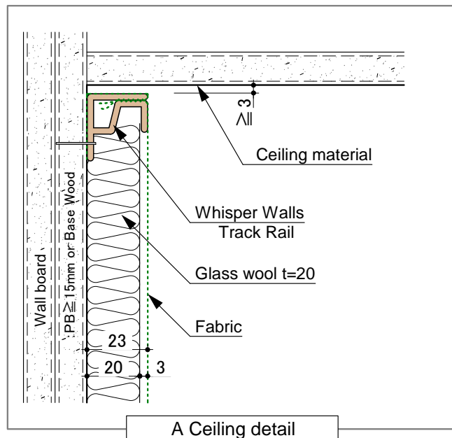
A Ceiling detail
