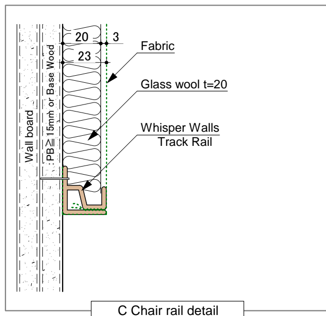
C Chair rail detail
