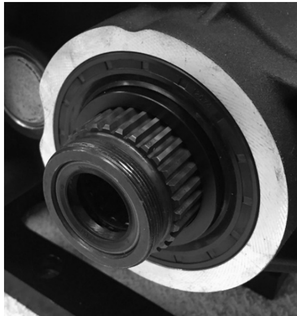
FIGURE 23 | MAIN DRIVE GEAR SEAL INSTALLED FLUSH WITH CASE
