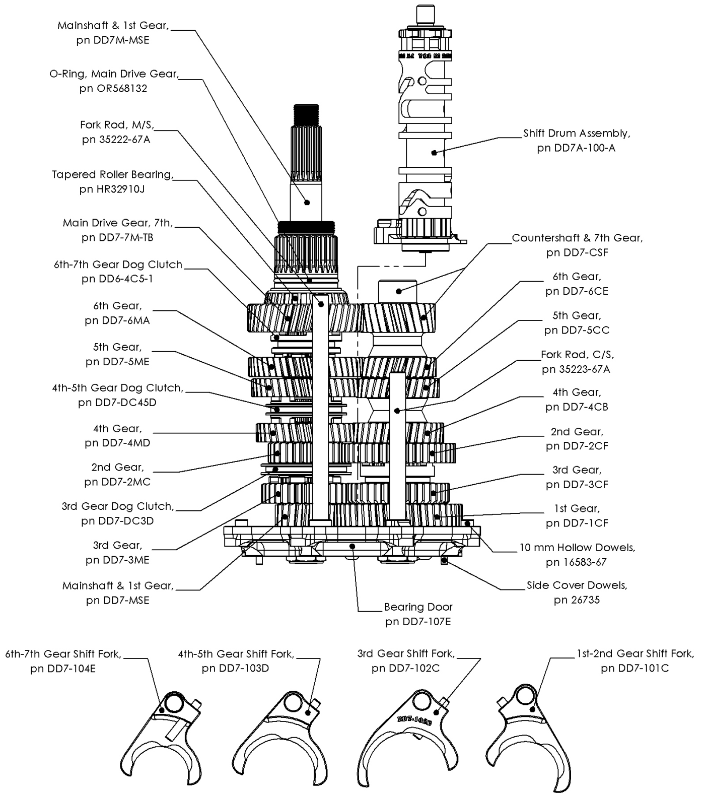
FIGURE 2 | GEARSET LAYOUT
