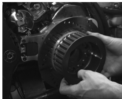
PULLEY AND ROTOR ASSEMBLY FIGURE 10
