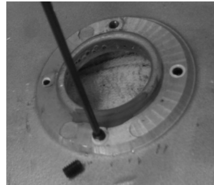
INSTALLING SET SCREWS | FIGURE 13
