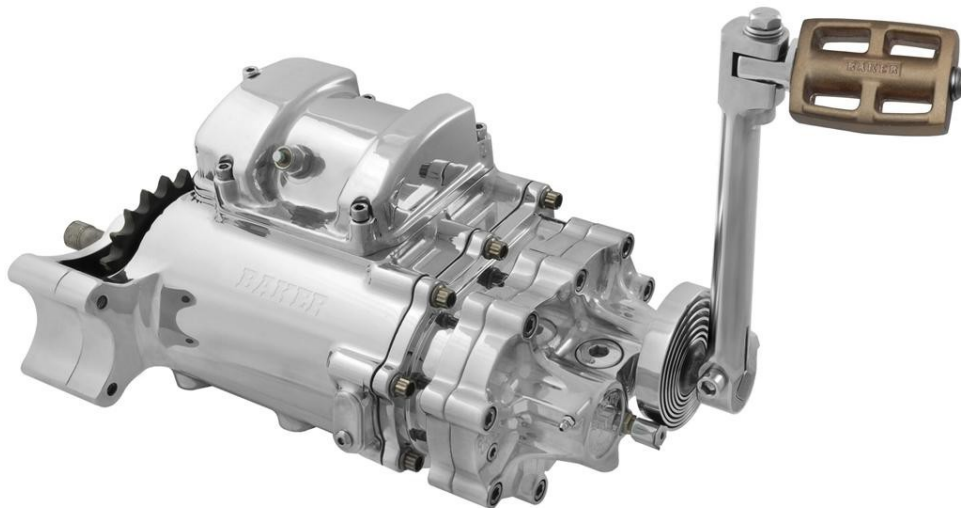
PN# 6N4-H002 (shown with bearing support)
