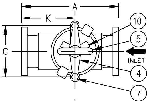
8" COVER & YOKE DETAIL
