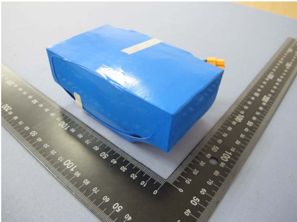
Fig.2 Overall view II of battery pack
