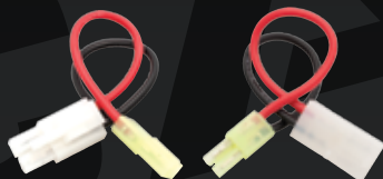
CHARGER ADAPTER LARGE TAMIYA MALE > MINI FEMALE MINI TAMIYA MALE > LARGE FEMALE
