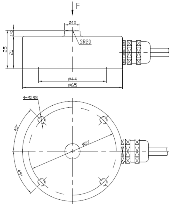
Dimensions (mm)
