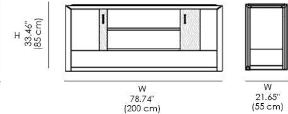
Sideboard With 2 Doors - 200
