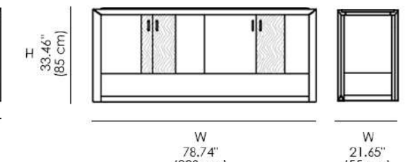
Sideboard With 4 Doors - 200
