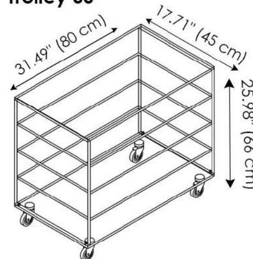
Grattacielo Fix 4-Tier Trolley 80
