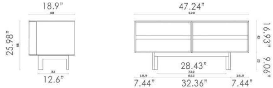
RAMBLAS Cabinet Design e-ggs BF 40 3 central glass shelf
