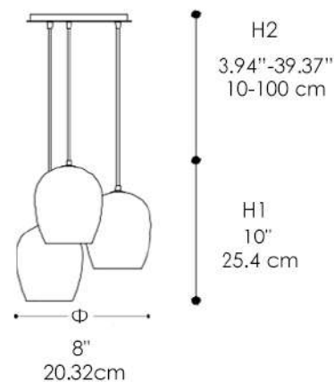
Nuce Pendant Lamp SL (4011/SL3)
