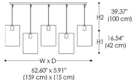
Mura Pendant Lamp (T1000/Comp. C)
