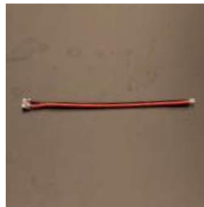
SPAC-JR-BASS-CABLE (Connecting Cable 2Pin) Wire gauge: 0.5mm 2 /20AWG Wire length: 15cm
