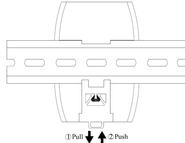
FIGURE 3: DIN-RAIL MOUNTING
