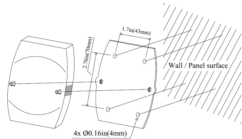
FIGURE 4: WALL/PANEL MOUNTING
