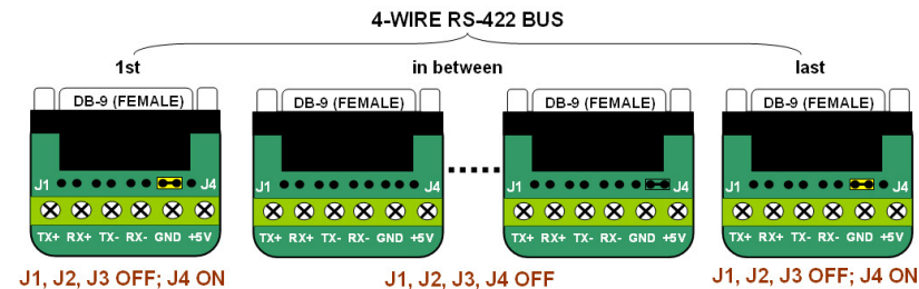
J1, J2, J3 OFF; J4 ON
