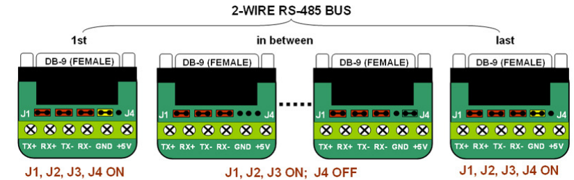
J1, J2, J3, J4 ON
