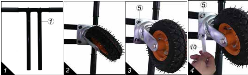
Step 2. Assemble the Attachment system to the foot plate frame
