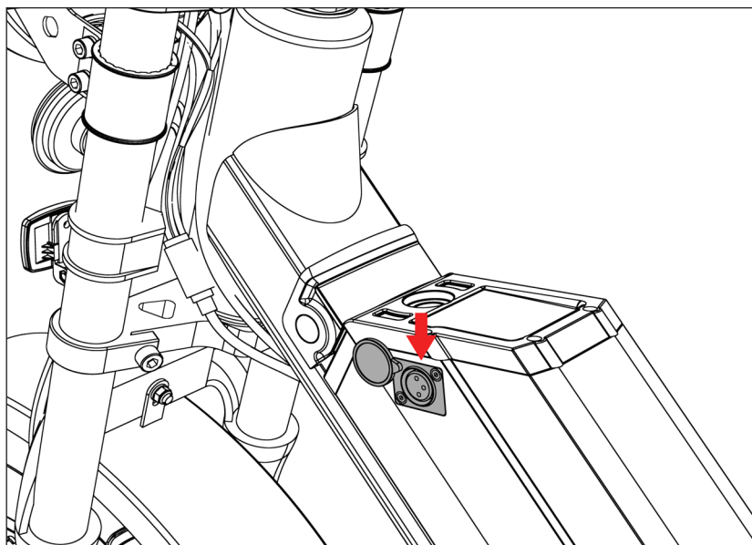
Fig. 28 - Charge Port
