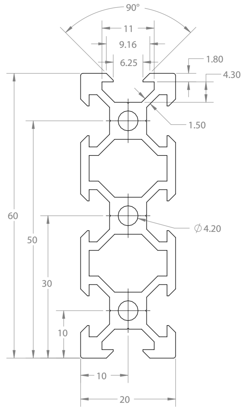
V-Slot 20X60 Linear Rail
