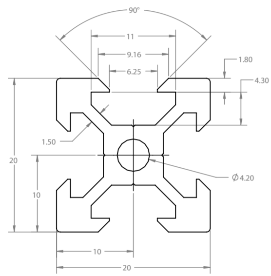
V-Slot 20X20 Linear Rail
