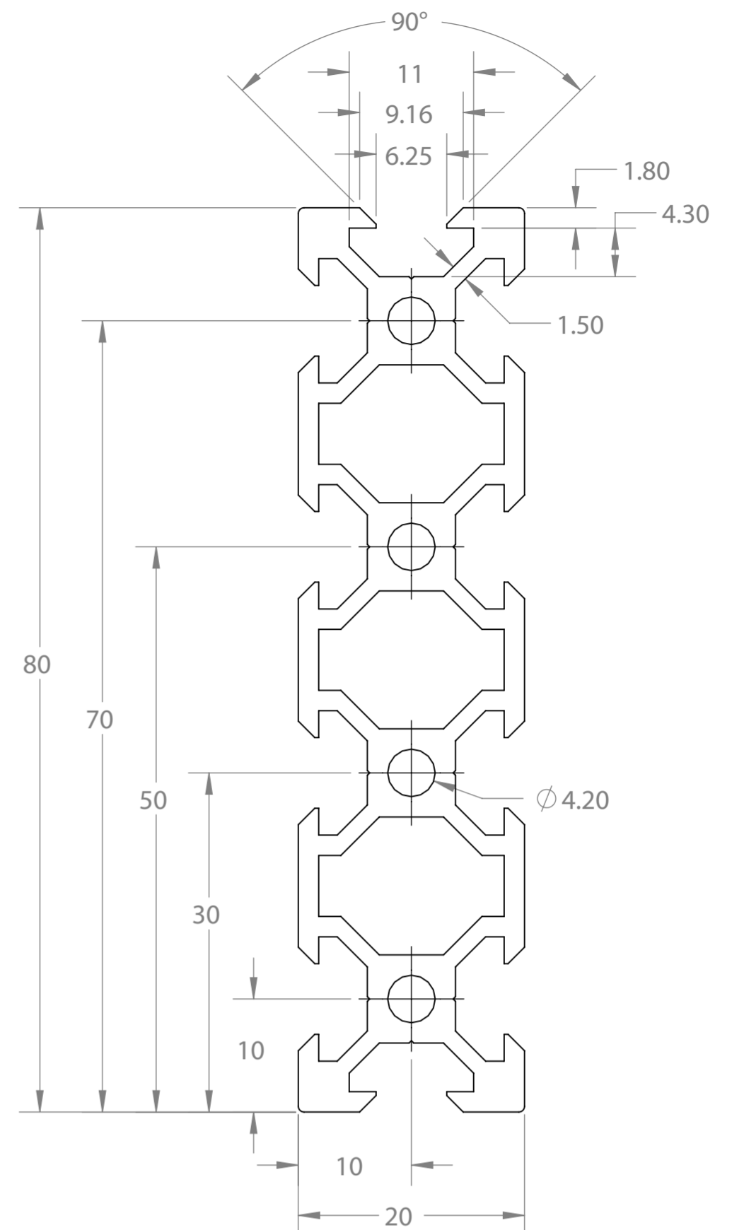
V-Slot 20X80 Linear Rail
