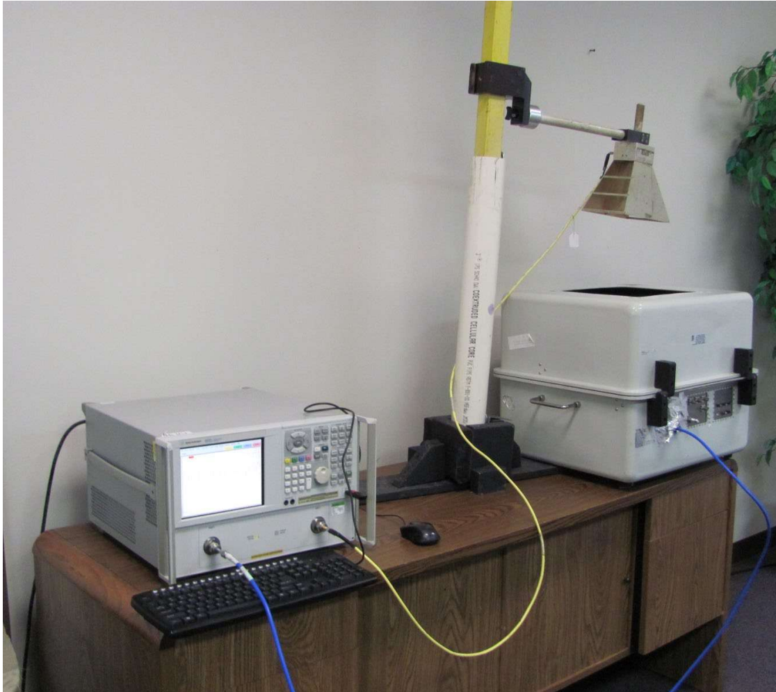
Figure 5. High Frequency Test Configuration Photograph – Above 6 GHz Testing
