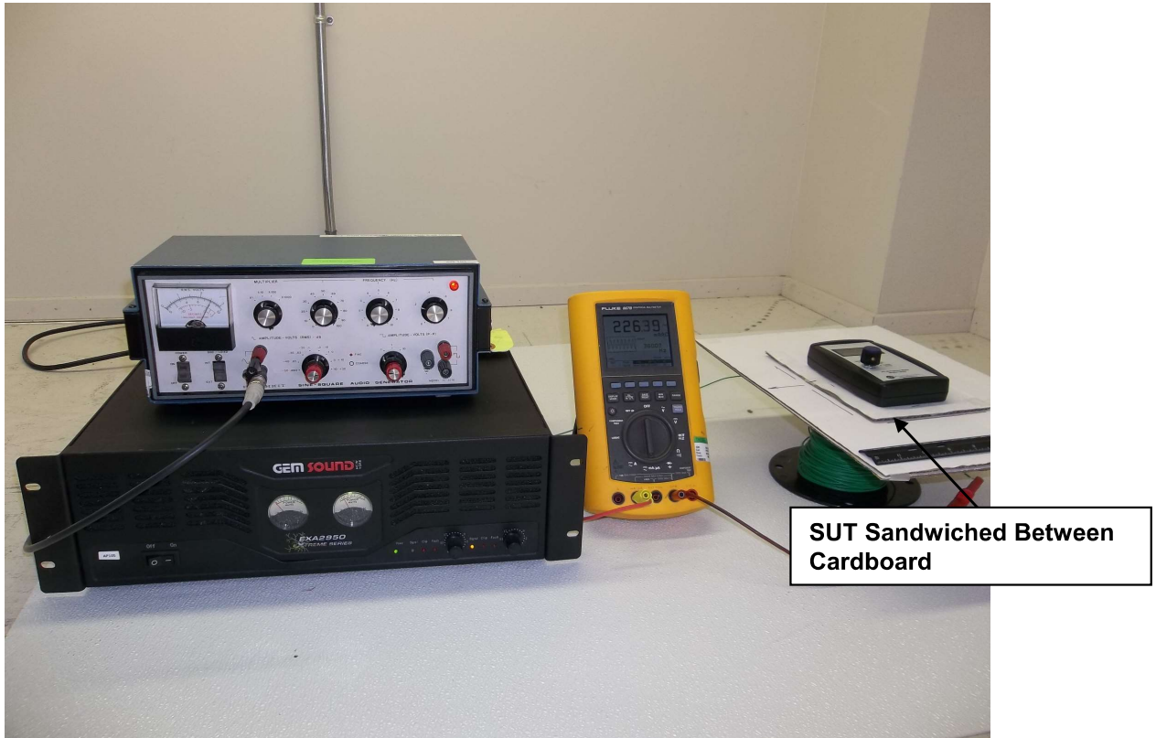
Figure 9. ELF EMR (Magnetic Component at 60 and 300 Hz) Test Configuration Photograph
