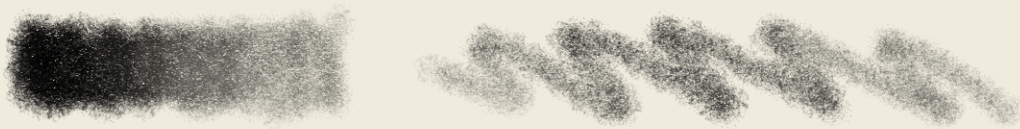
Blendy Shader
