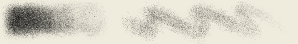
Noise Shader
