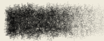
Soft Shader
