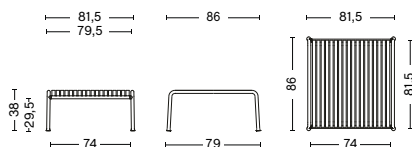
PALISSADE LOW TABLE LENGTH 81,5 CM | 32" WIDTH 86 CM | 33.75" HEIGHT 38 CM | 15"
