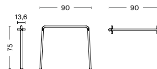
PALISSADE MIDDLE LEG WIDTH 90 CM | 35.50" DEPTH 13,5 CM | 5.25" HEIGHT 75 CM | 29.50"
