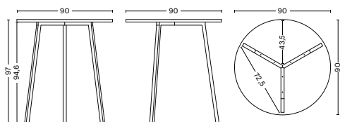
LOOP STAND HIGH ROUND | Ø90 DIAMETER 90 CM HEIGHT 97 CM TABLETOP THICKNESS 2,4 CM
